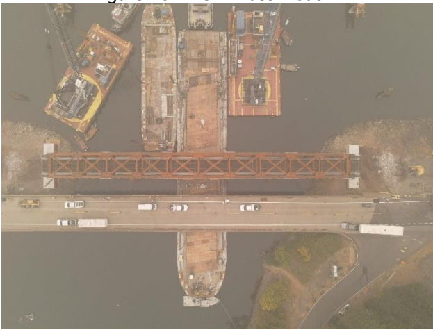
Figure 11 - New Truss Float In
