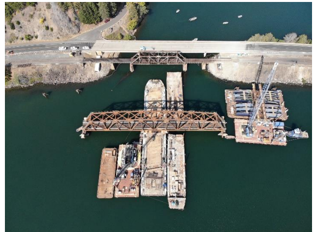
Figure 7- Float In Configuration
