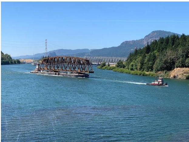
Figure 6 - Truss Transportation
